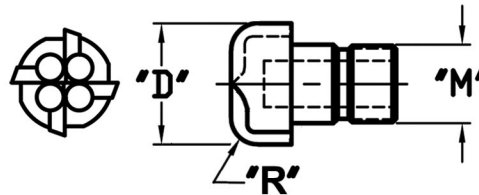
CORNER RADIUS FOAM CUTTER HEADS
