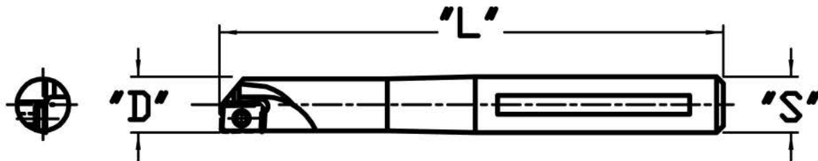
Available With 1/16" or 1/32" Insert Radius
