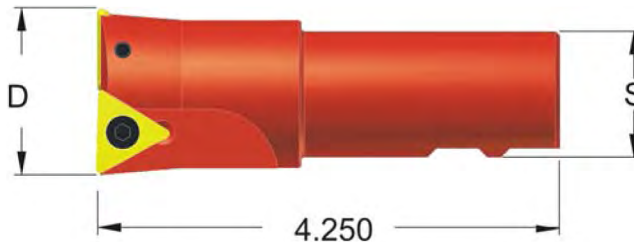
WELDON FLATS SPOT FACER TOOL
